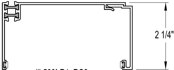
#L500I-R1, RC2 FOR 3 3/4" WINDOW SYSTEMS
